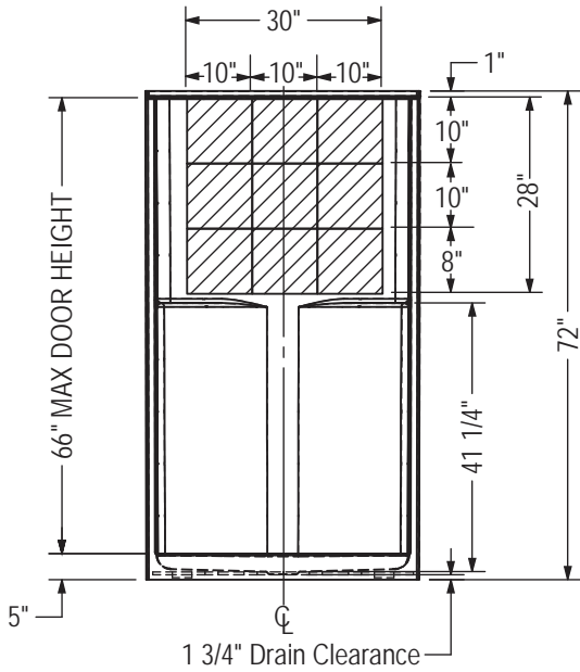
BACK WALL Reinforcement
