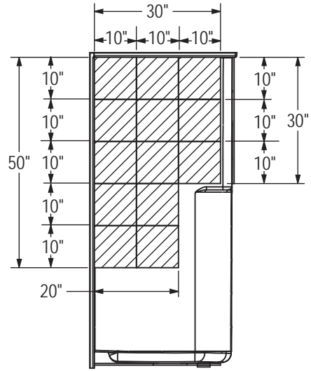
SIDE WALL Reinforcement
